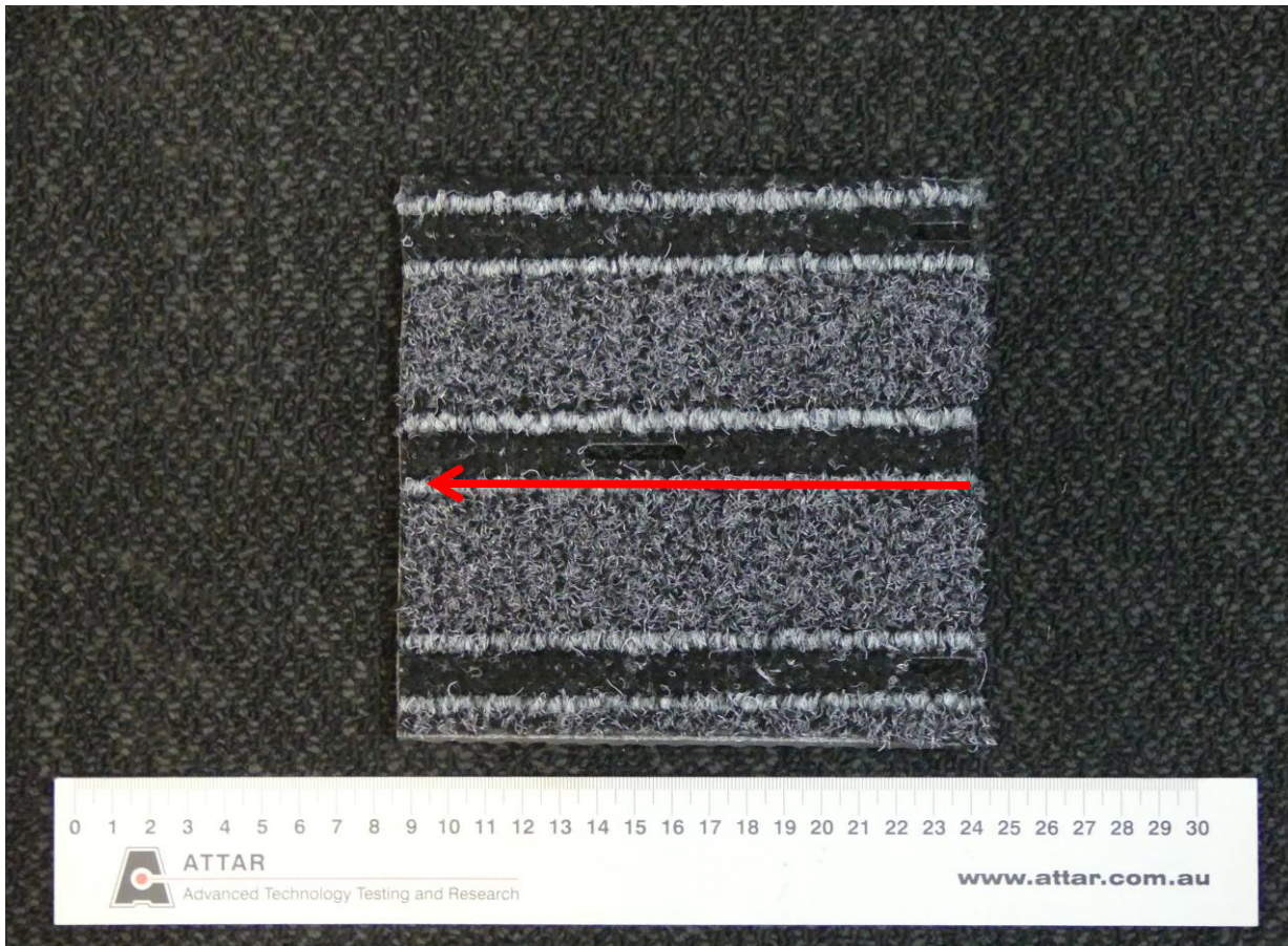
Figure 1: Romus Scrapex Arrow indicates direction of testing
